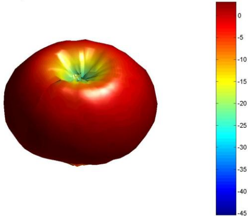
3D radiation at 2.4GHz.jpg
