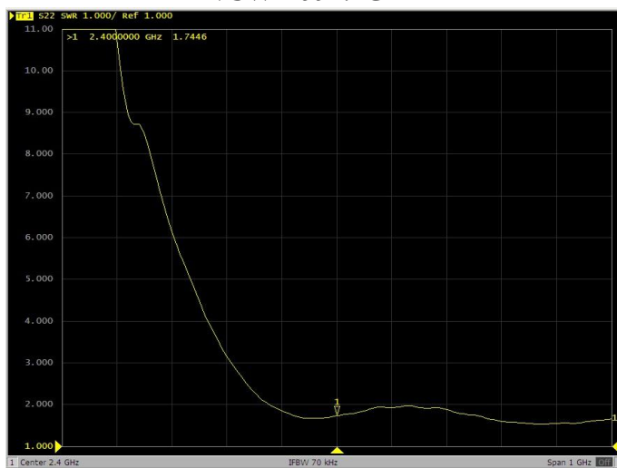
VSWR at 2.4GHz
