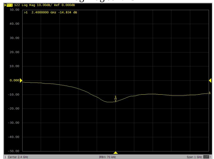
Log Mag at 2.4GHz
