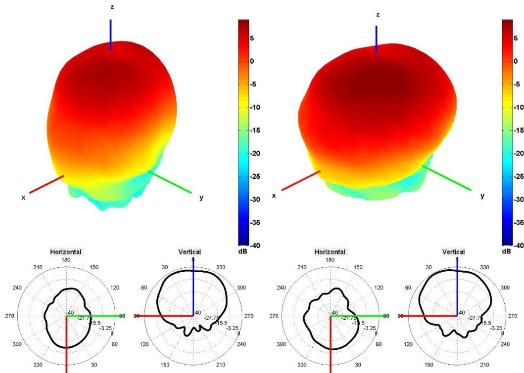
2350 and 2600 MHz Radiation pattern
