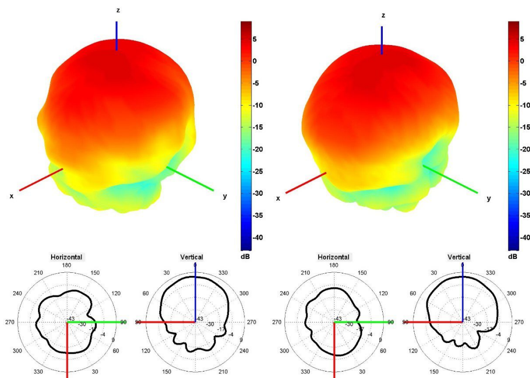
1500 and 1600 MHz Radiation pattern
