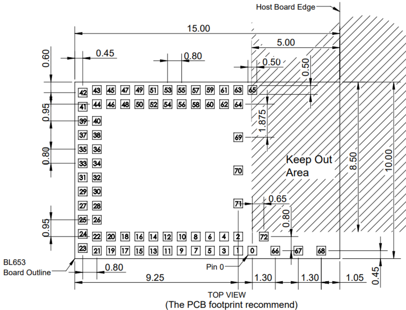
Figure 20: Land pattern and Keep-out for the 453-00039
