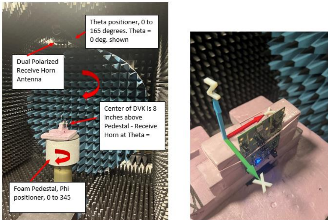
Figure 8: Radiated Performance Measurement Setup
