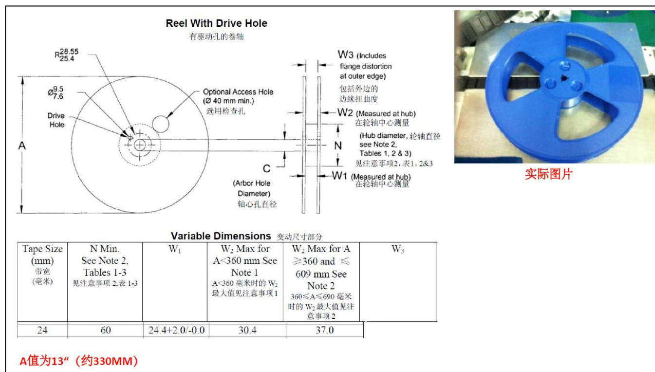
Figure 21: Reel specifications
