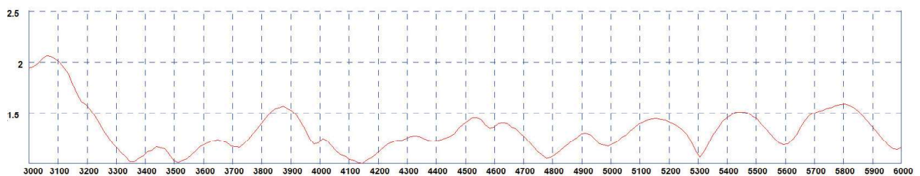
Typical VSWR*
