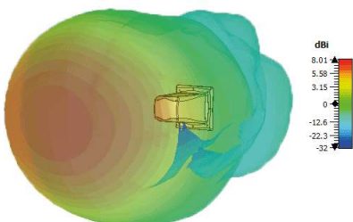
Typical 3D Pattern 5.4GHz**
