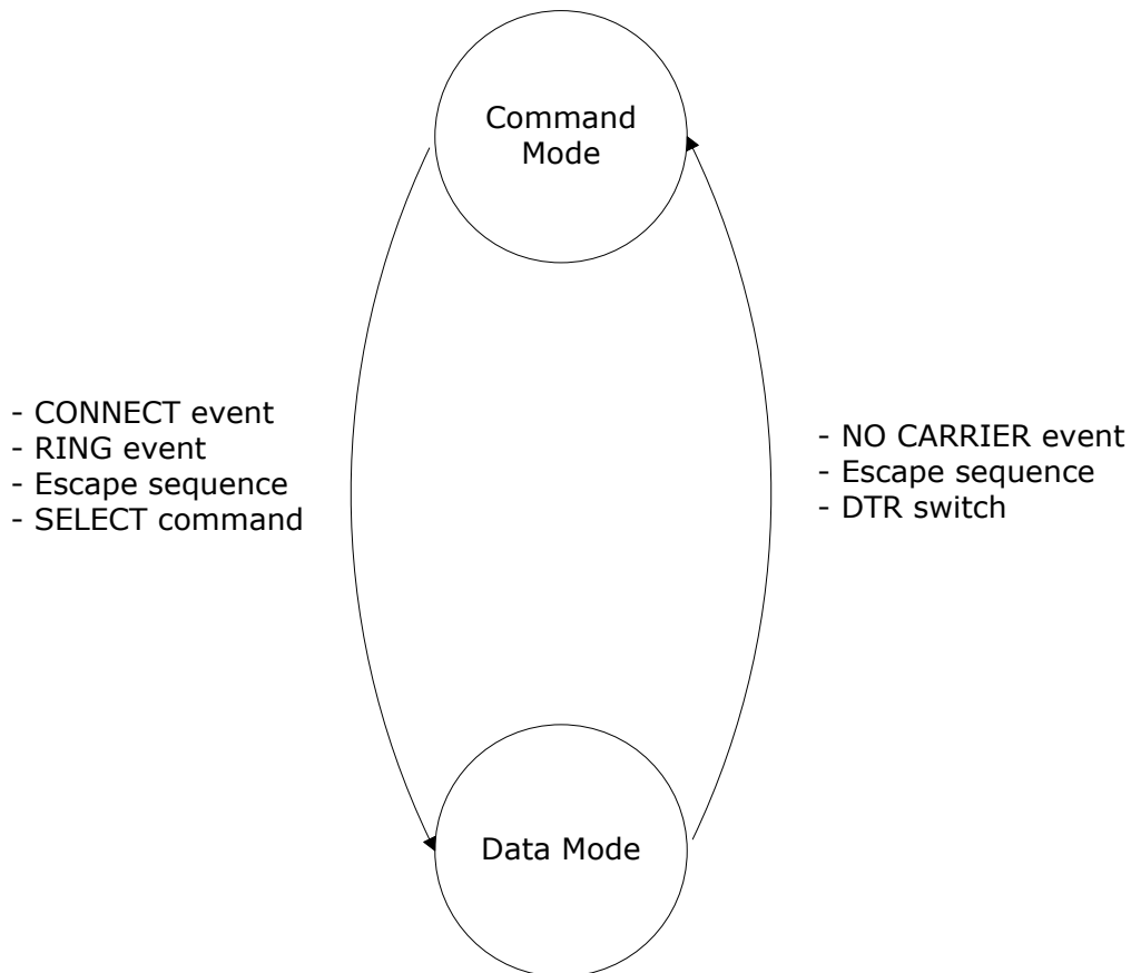
Figure 7: Mode transitions
