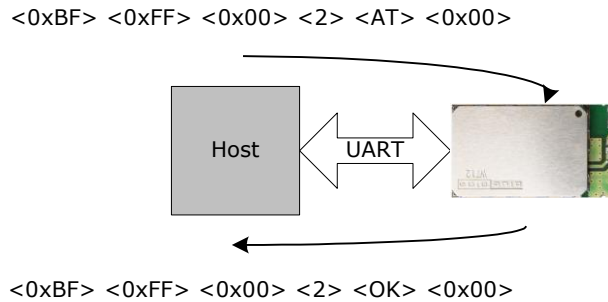
Figure 9: Host-iWRAP-Host communication
