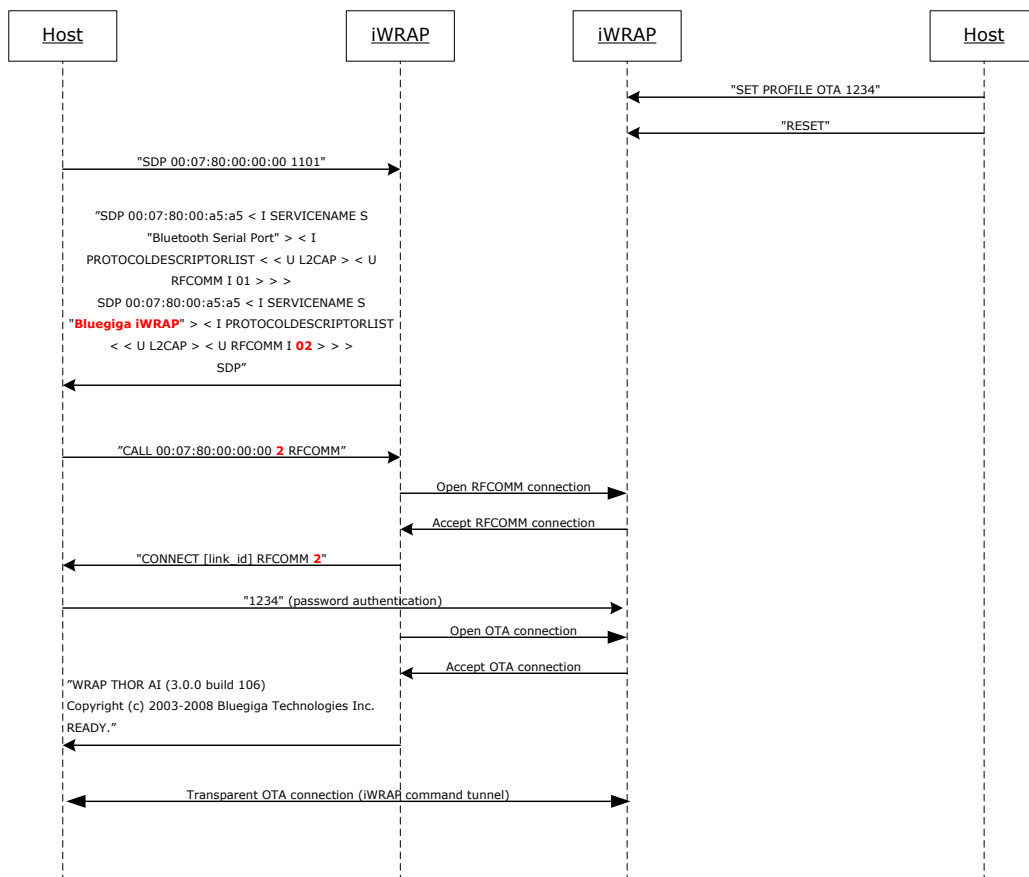
Figure 17: Over-the-Air connection example
