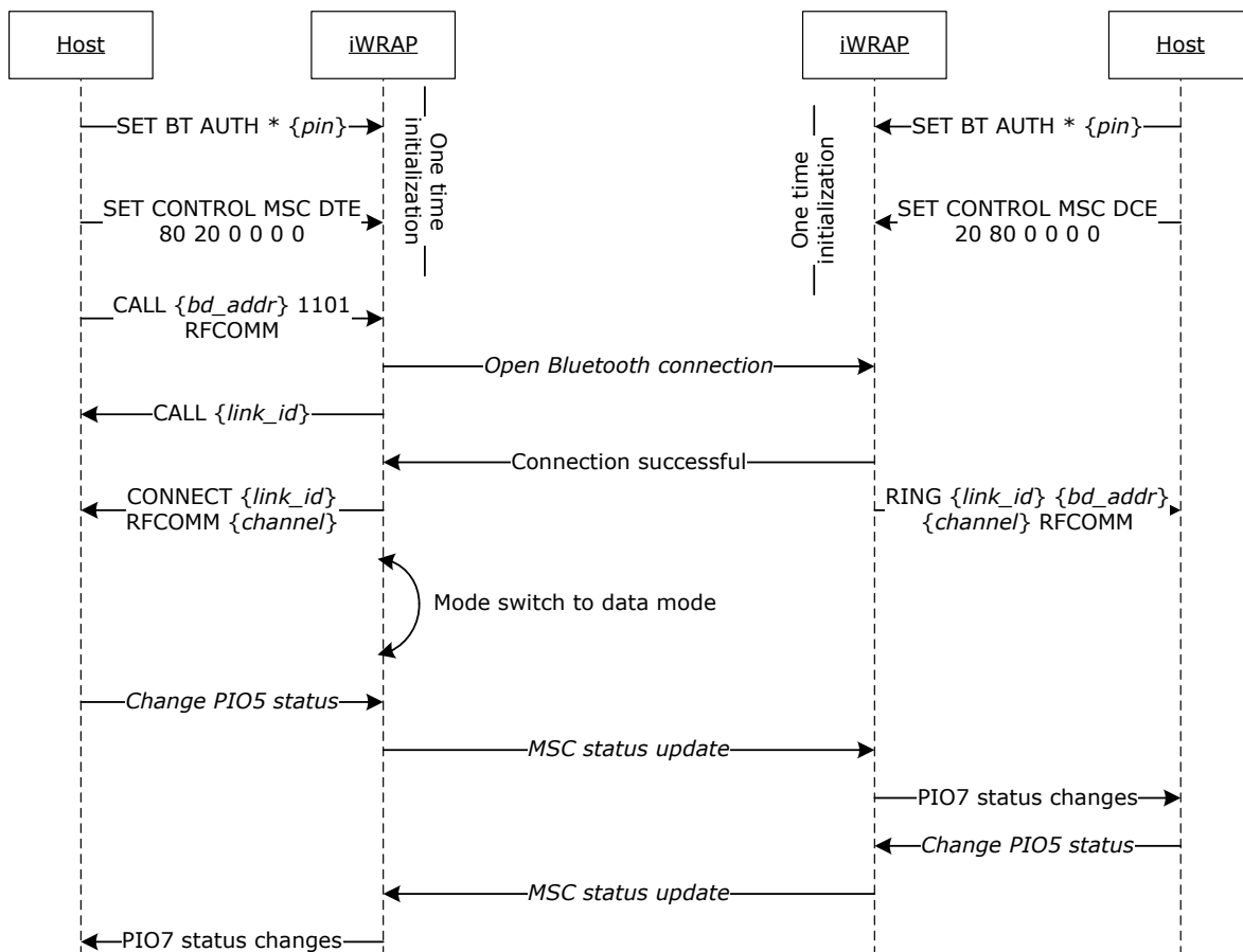
Figure 15: Wireless IO replacement connection
