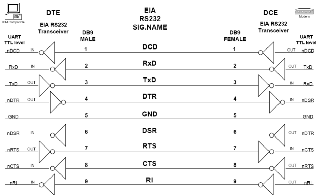
Figure 12: RS232 connections
