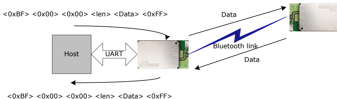
Figure 10: Host-iWRAP-remote device communications
